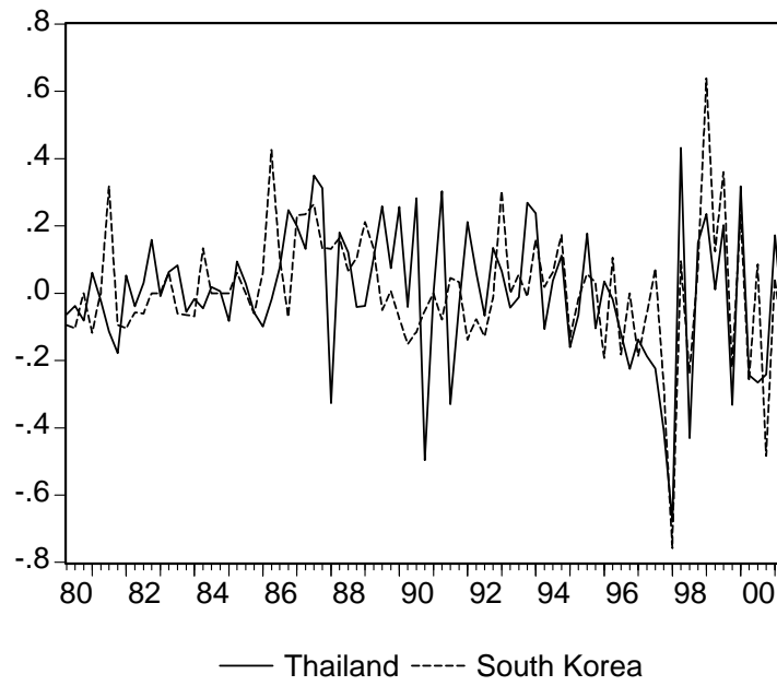
Figure 1: Quarterly Returns for Thailand and South Korea
