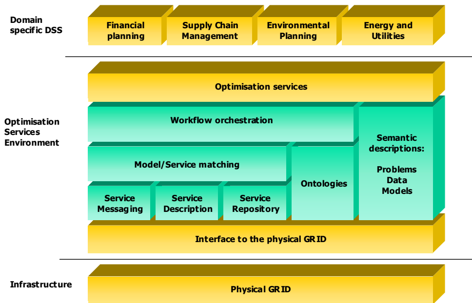
Figure 6. Virtual organisation for optimisation services
